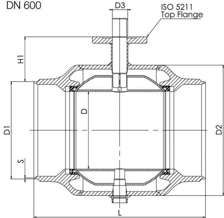
DN 600
